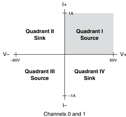
Figure 1. PXIe-4112 Quadrant Diagram
